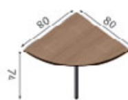
DK-01 linking unit
